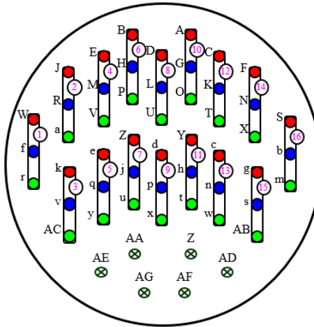
Male wiring side / Female testing side
