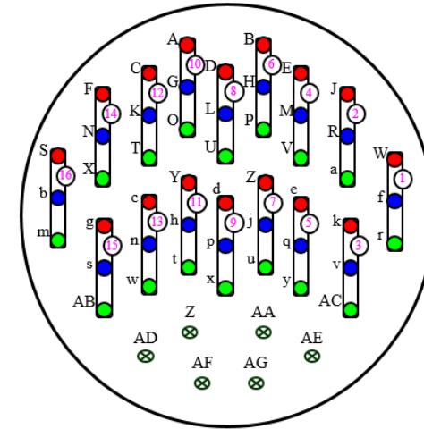
Female wiring side / Male testing side
