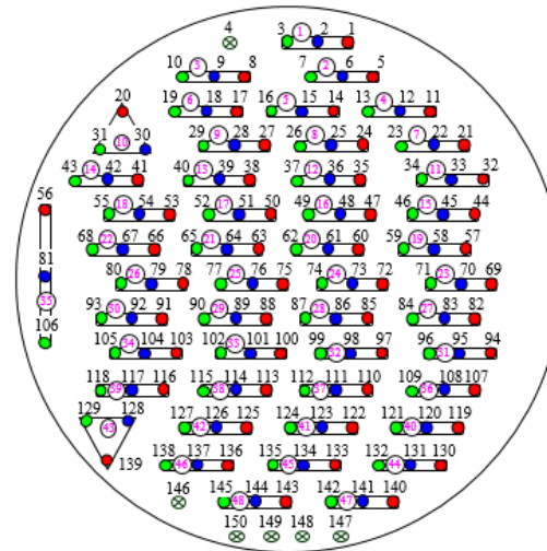
Male wiring side / Female testing side
